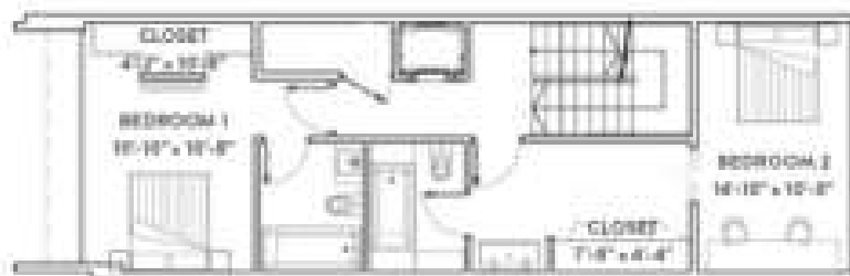
LEVEL 2
